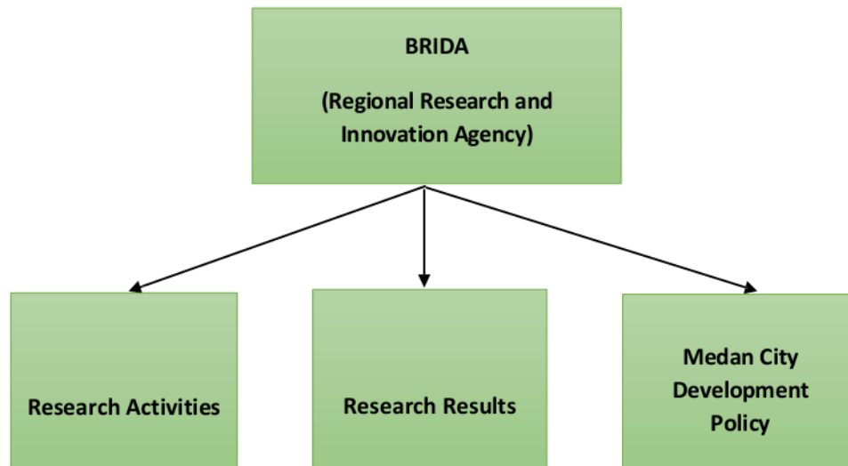
Figure 1. Thinking Framework
